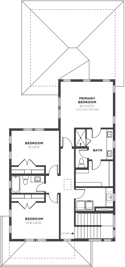
SECOND FLOOR
