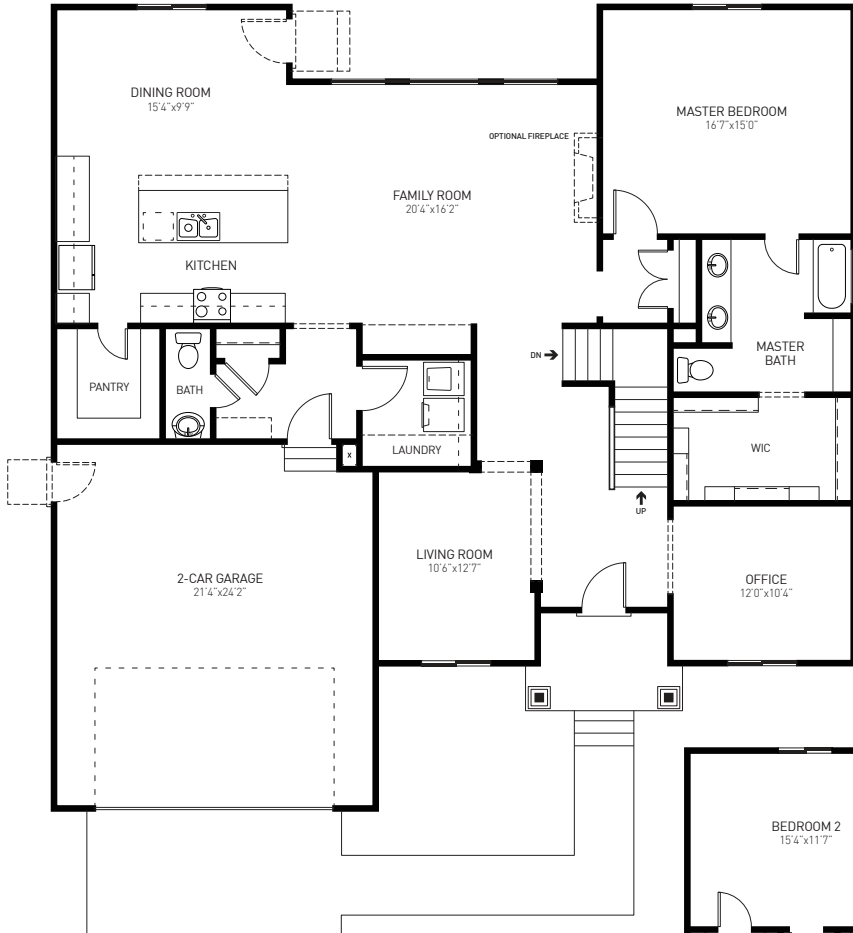
MAIN FLOOR
