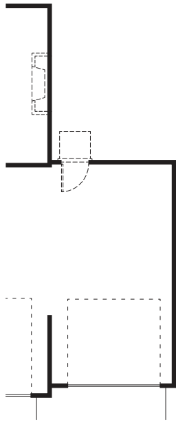
OPTIONAL 3-CAR GARAGE (12'x22')
