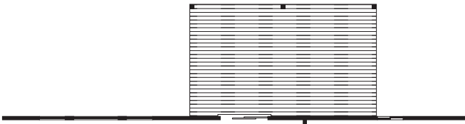
OPTIONAL DECK (12'x20')
